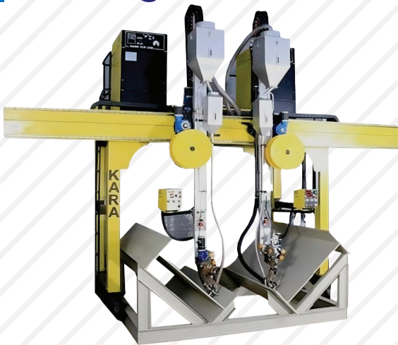
■ Gantry Welding Machine Submerged welding (KAW.TB)
